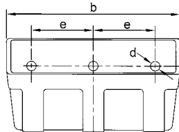
Plastic elevator buckets type D (parameters in mm)
