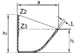
Plastic elevator buckets type D (parameters in mm)
